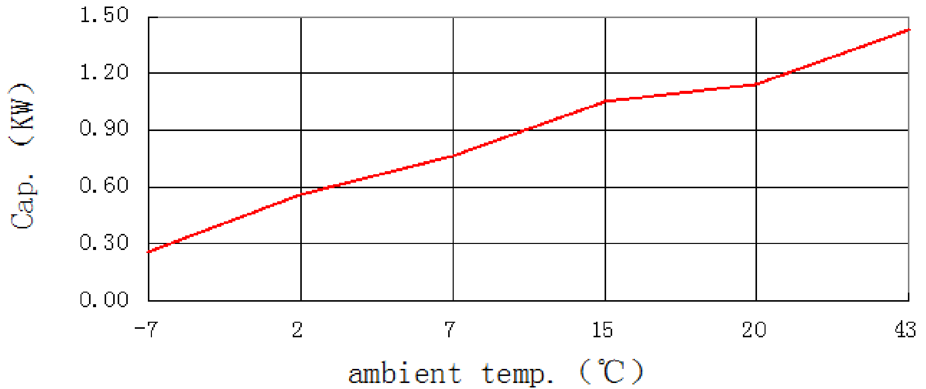
capacity curve
